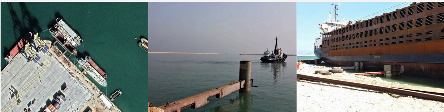
MOORING PILES AT TRIPOLI COMMERCIAL PORT
